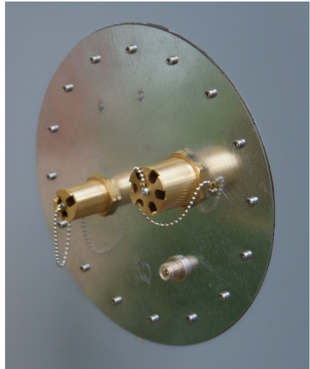
3 and 6 couples fiber optics feedthrough for 9GHz cut-off frequency
