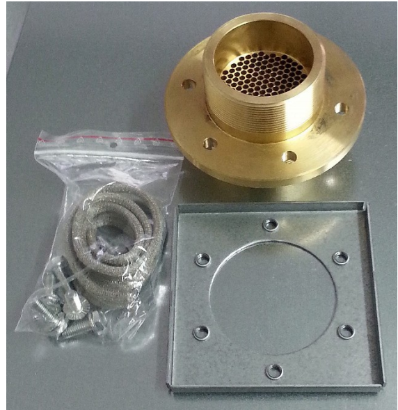
Gas or liquid waveguide 20GHz
